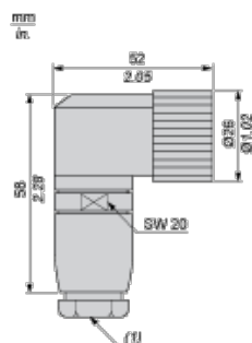
(1) Cable gland: no. 13 metal (Pg 13.5)
