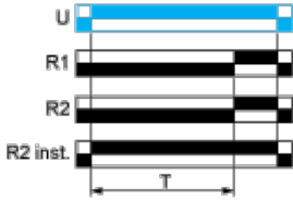
Function: 2 Outputs
