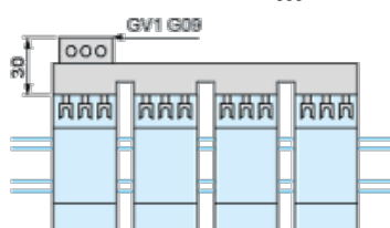
Sets of Busbars GV2G245, GV2G254, GV2GR272
