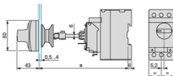
Door cut-out
