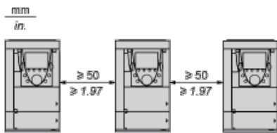
Type B Mounting
