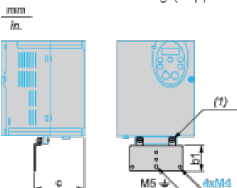
Plate for EMC mounting (supplied with the drive)
