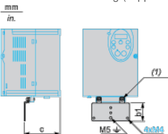
Plate for EMC mounting (supplied with the drive)
